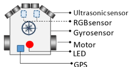
Figure 4: ROBOT configuration
